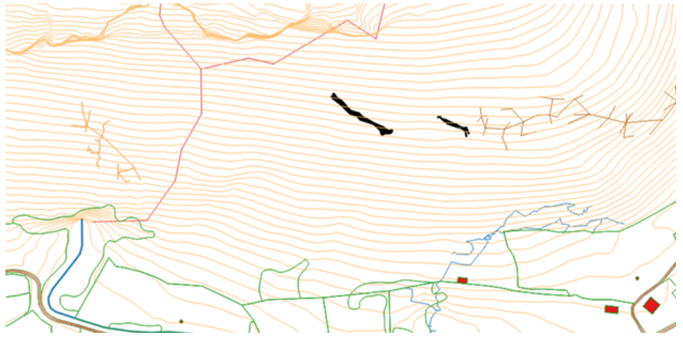
Relative positions of 0061 (left) and 1294 (right), with partial line surveys of Cueva del Agua (red), Cueva Sotarraña (orange), Cueva Cofresnedo (brown) and Cueva de los Tizones (blue)
