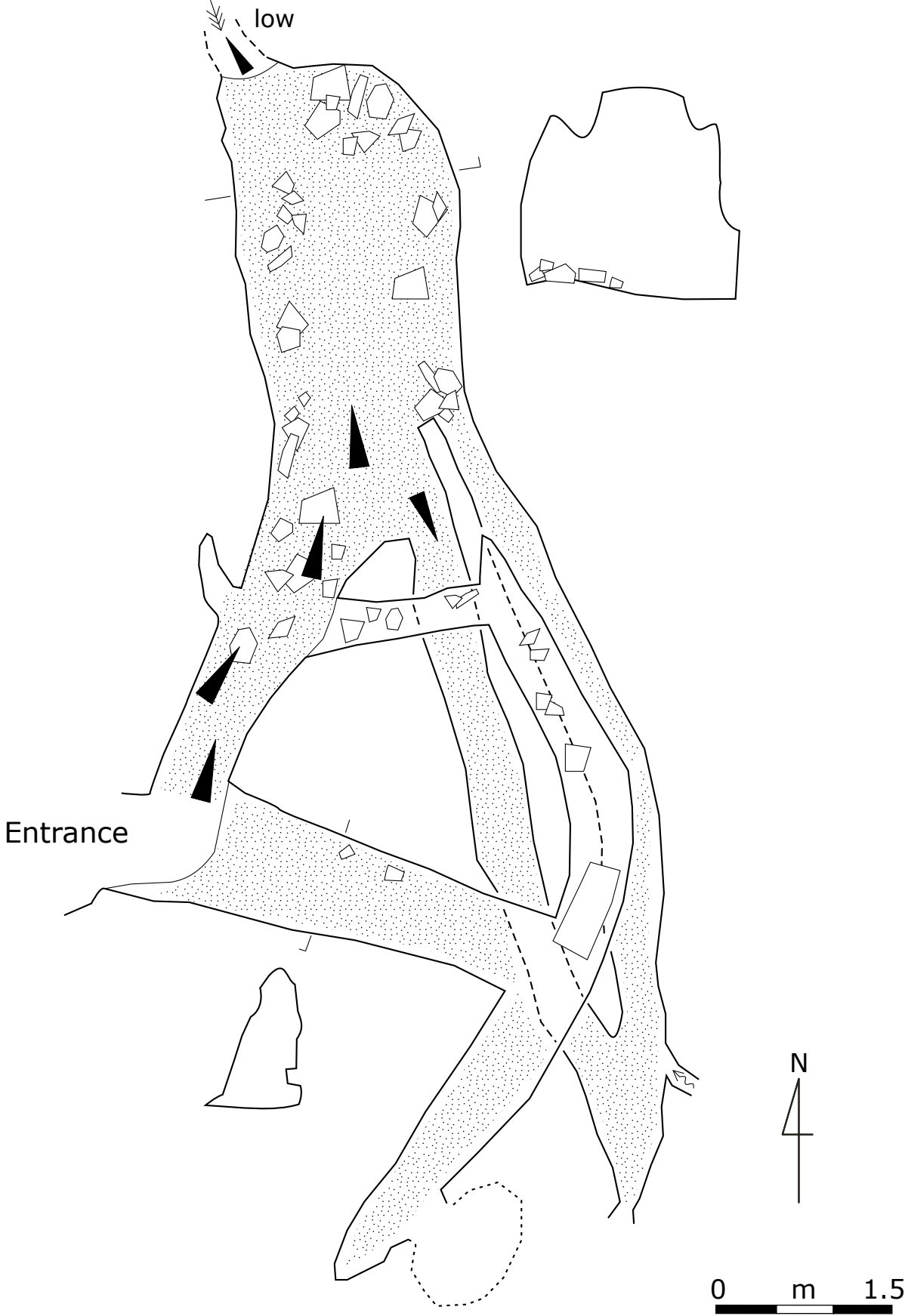
Cueva de la Puerta (0024) Ozana, Matienzo. Length 34m 453528 4795371 210m July 2024 Surveyed and drawn: PS
