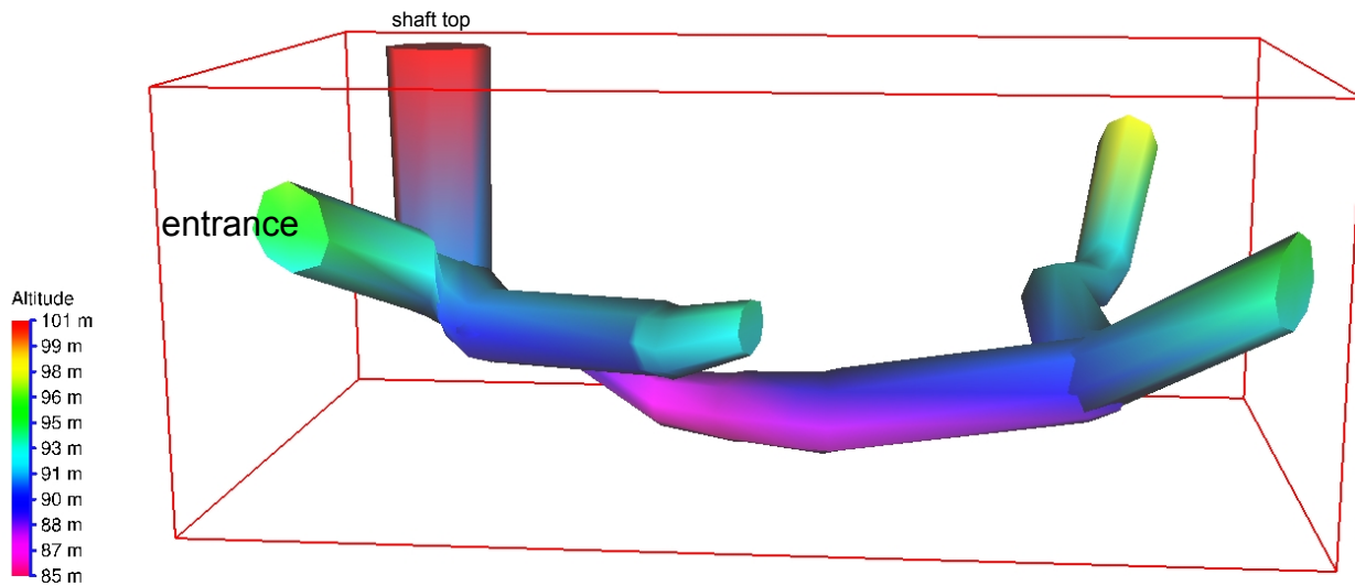
PROJECTED SECTION on 265° - 85° (auto passage widths from Loch application)
