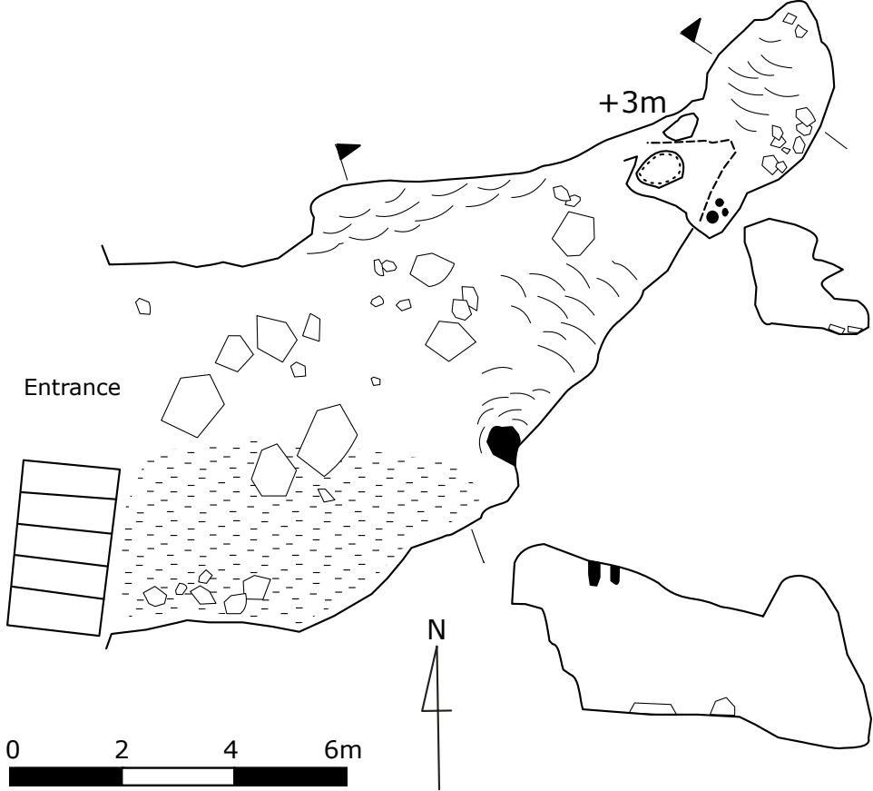
Cueva 1455 Cubija, Matienzo 450193 4796712 268m Length 18m Surveyed Nov. 2020 PS
