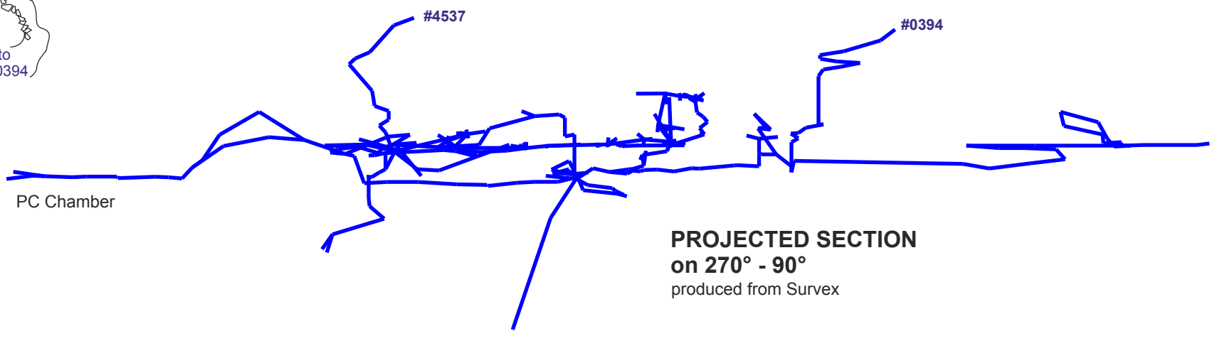
PROJECTED SECTION on 270° - 90° Eastwater entrance section
