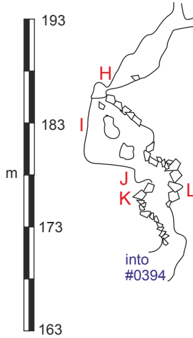
PROJECTED SECTION on 270° - 90° Eastwater entrance section
