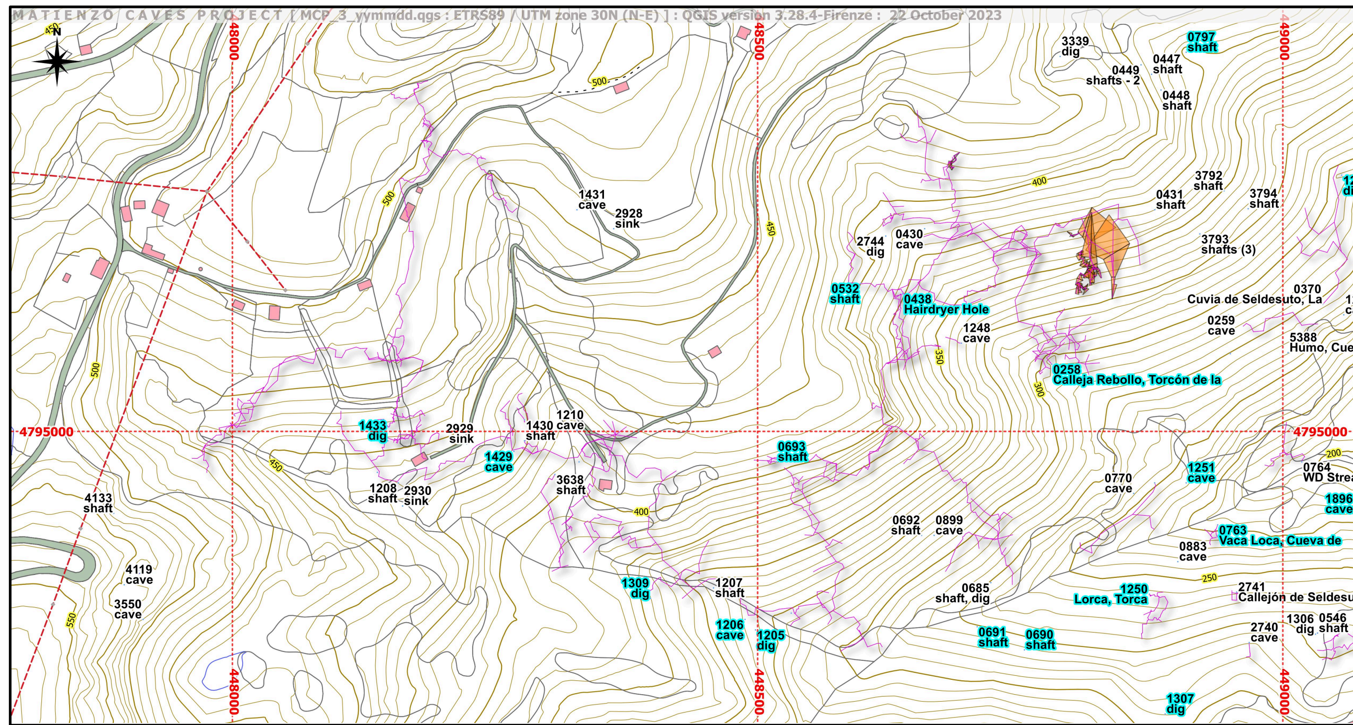
Map showing the centre line of Toad in the Hole with other centre lines and entrances in the vicinity
